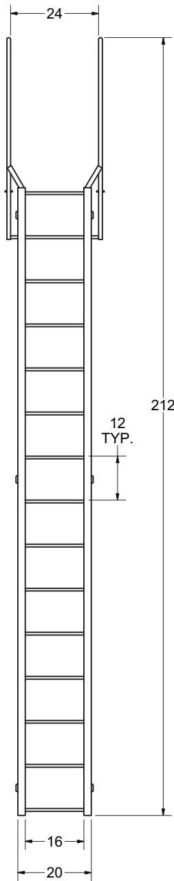
DETAIL A
